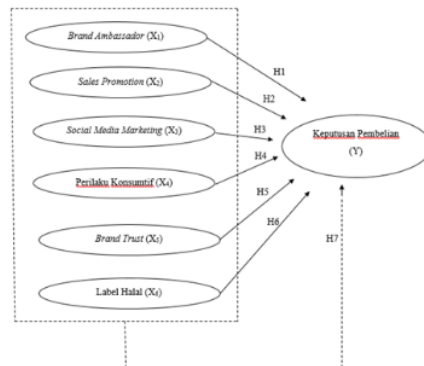
Gambar 1. Model Penelitian
