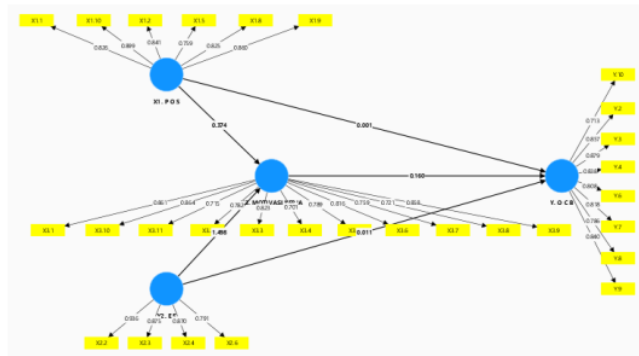
Gambar 4. F-Square
