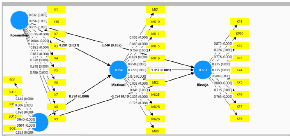
Gambar 3 Path Coefficient
