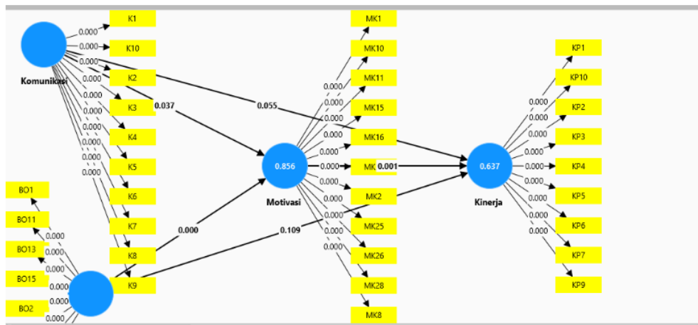
Gambar 2 Inner Model
