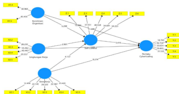
Sumber: Output SmartPLS, 2024
